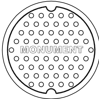
D & L #K-6313 STREET MONUMENT RING & COVER OR APPROVED EQUAL LABELED "MONUMENT"
