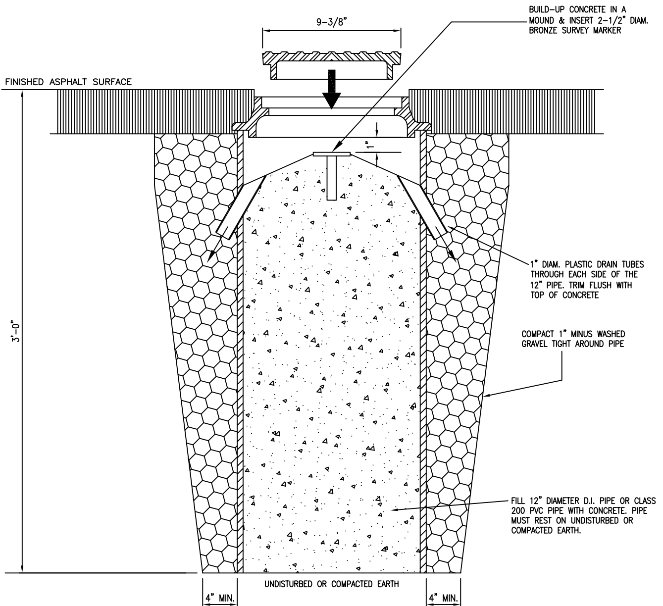
D & L #K-6313 STREET MONUMENT RING & COVER OR APPROVED EQUAL LABELED "MONUMENT"
