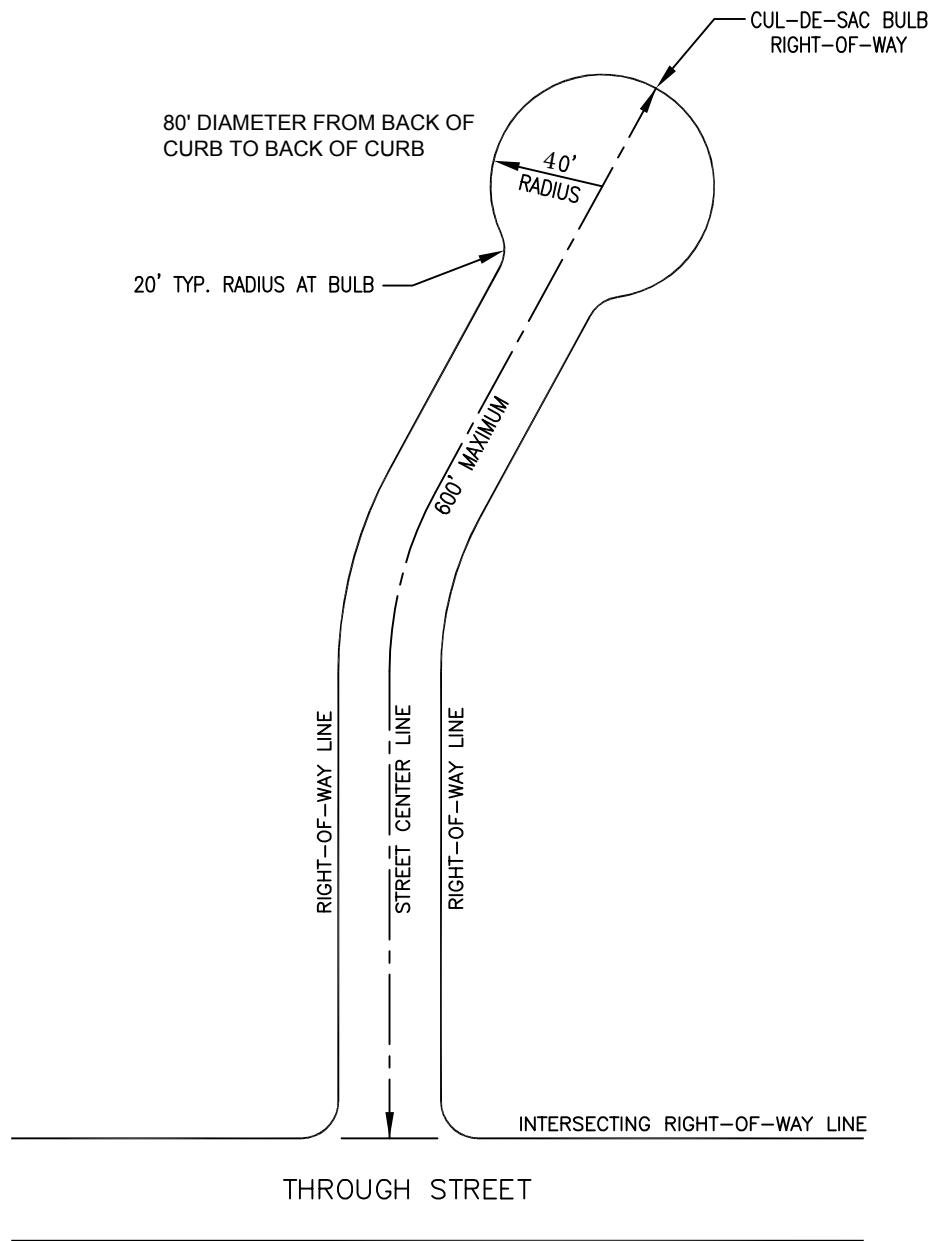
MINIMUM & MAXIMUM CUL-DE-SAC LENGTHS
