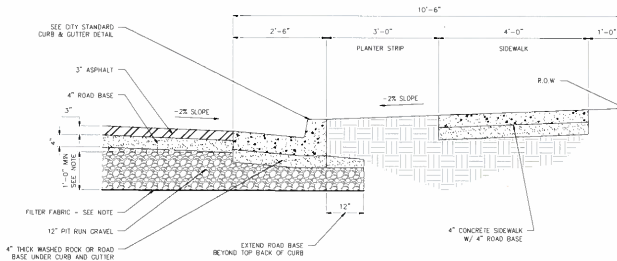
LOCAL - 50' RIGHT-OF-WAY PAVING MATERIALS
