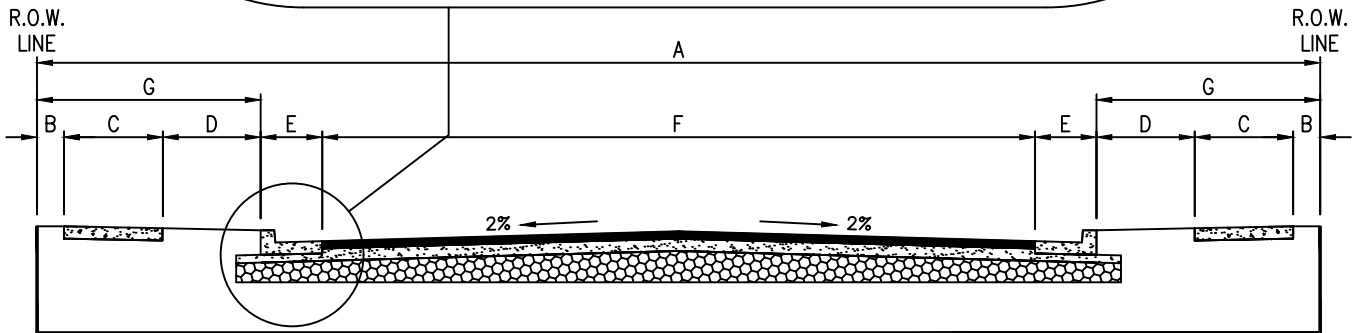
TYPICAL STREET CROSS-SECTIONS
